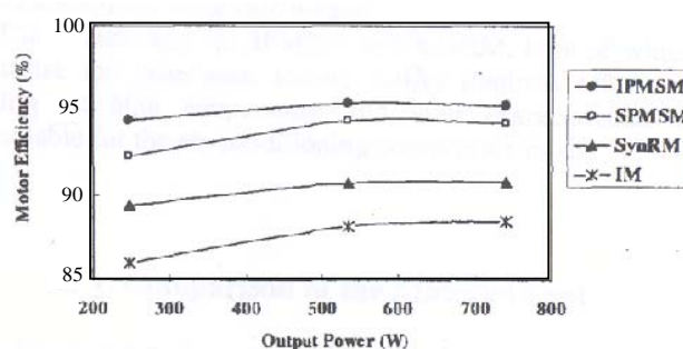
Fig. 8. Motor efficiencies at 4000r/min.
